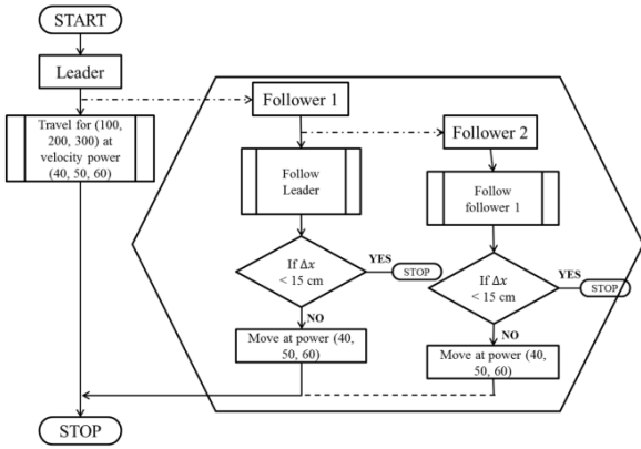
Figure 2: Algorithm flow
